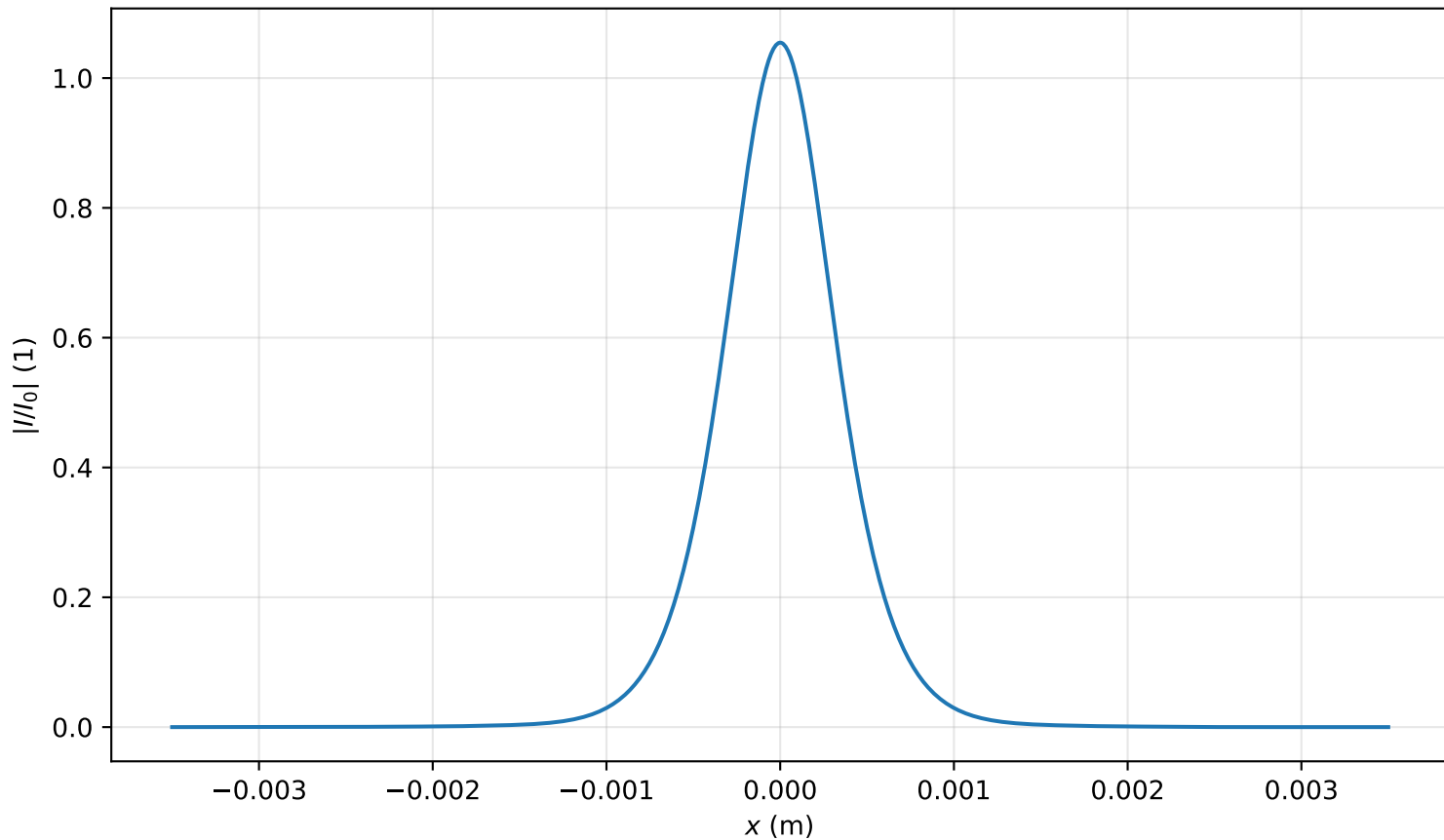
Intensity profile I(x, y = 0, z = 3.184m)/I_0 , P_{in}=0.8P_{cr} , artificial time
